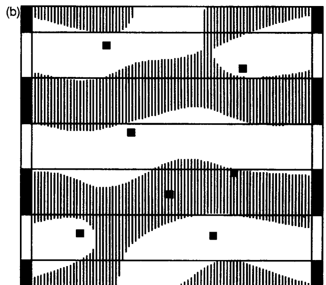
Figure 4(b). A non-plane wave of a different wavelength can produce exactly the same amplitudes and phases at all stations of the network. This wave is composed of nine plane waves of wavelength 1.2\lambda , all propagating within \pm 45^\circ of the original direction of propagation.
